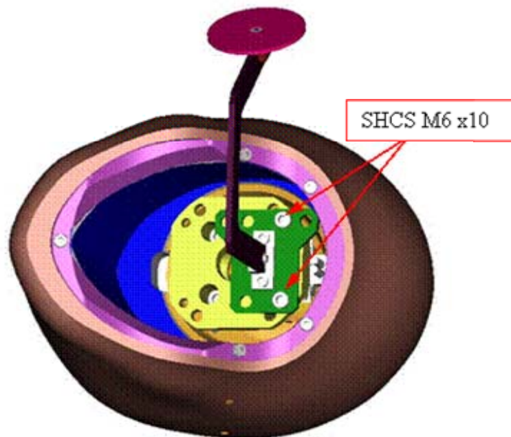
Figure 3 — Head bracket installation for lateral drops
